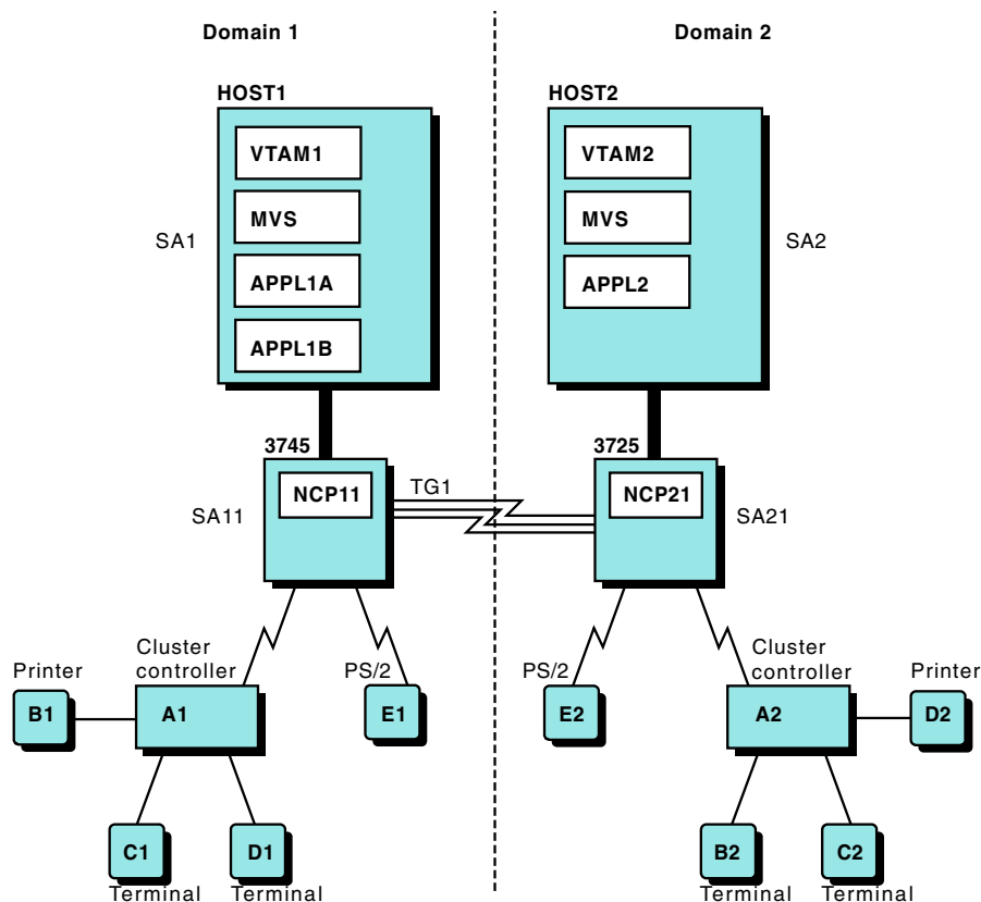
Figure 138. Multiple-domain network
