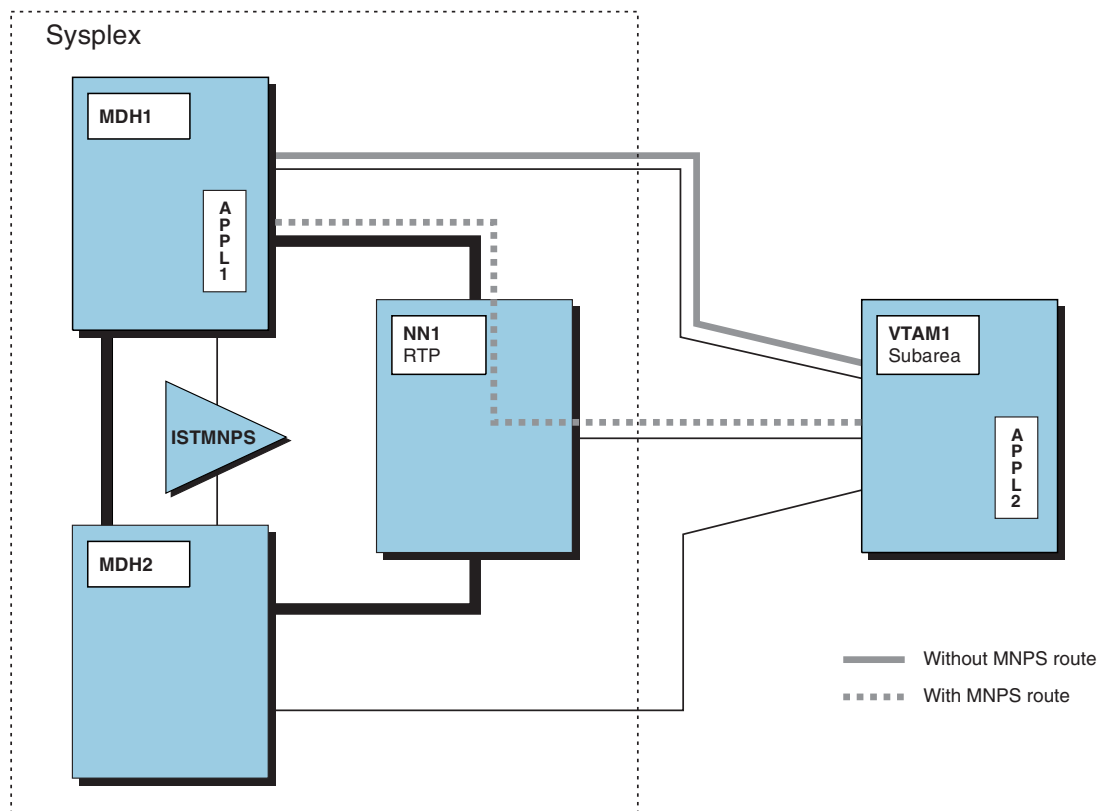
Figure 116. Session routes
