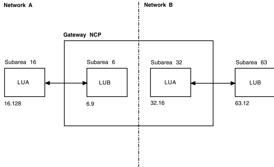
Figure 151. Address translation
