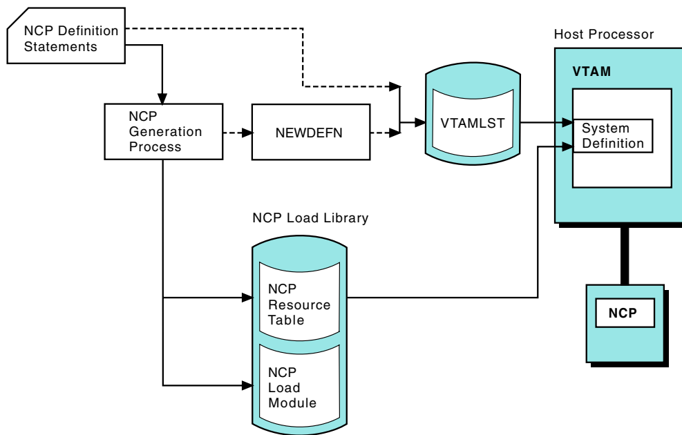
Figure 156. NCP generation
